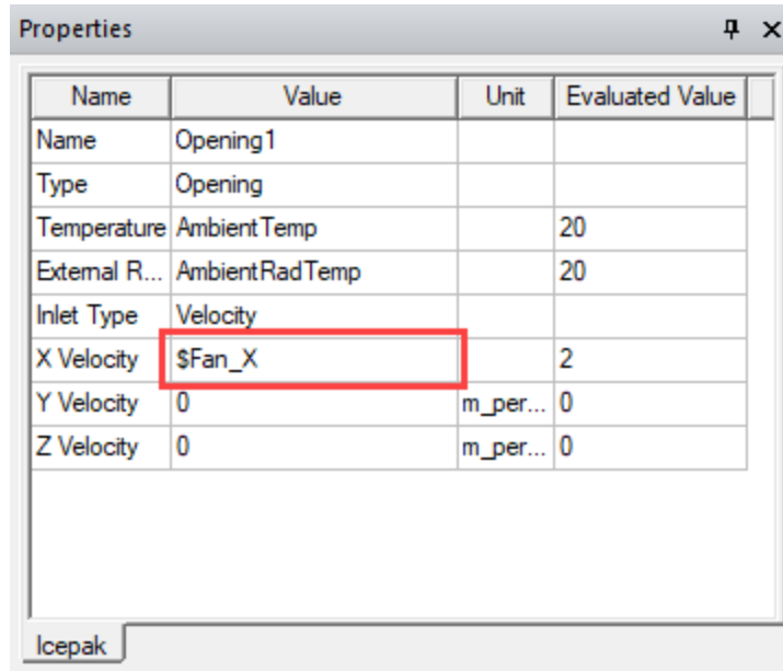
Figure 6-5: Opening1 properties with variable
