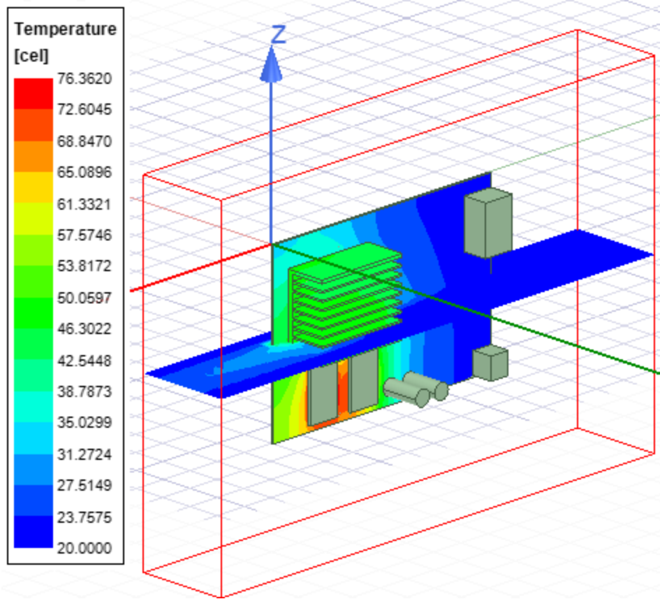
Figure 4-15: Temperature contours on a plane
